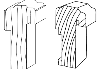
1-3/4" ASTRAGAL
